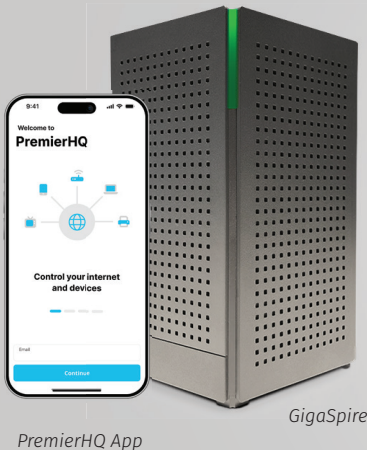
PremierHQ App
